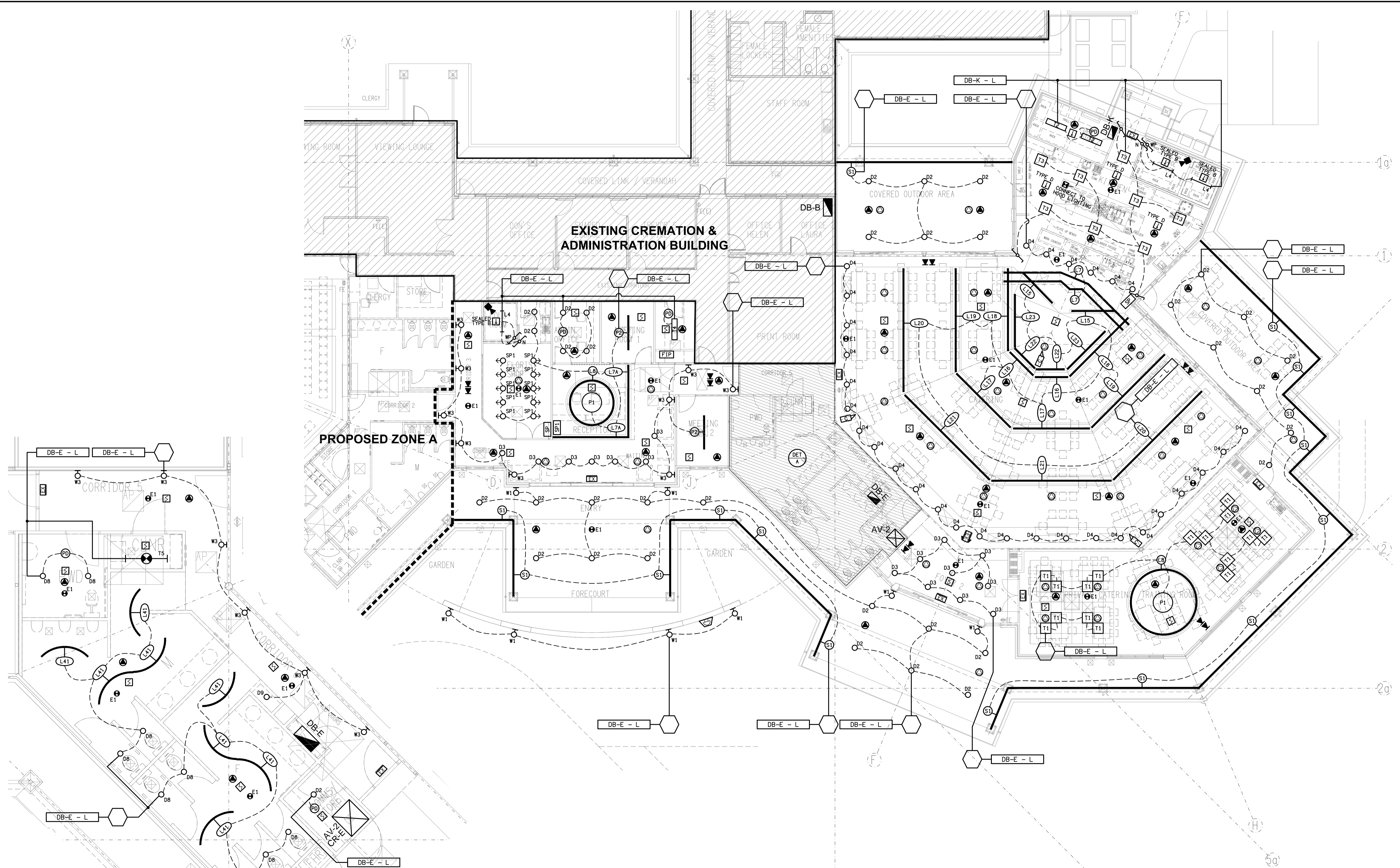
DETAIL A AMENITIES REFLECTED CEILING PLAN SCALE 1:50
